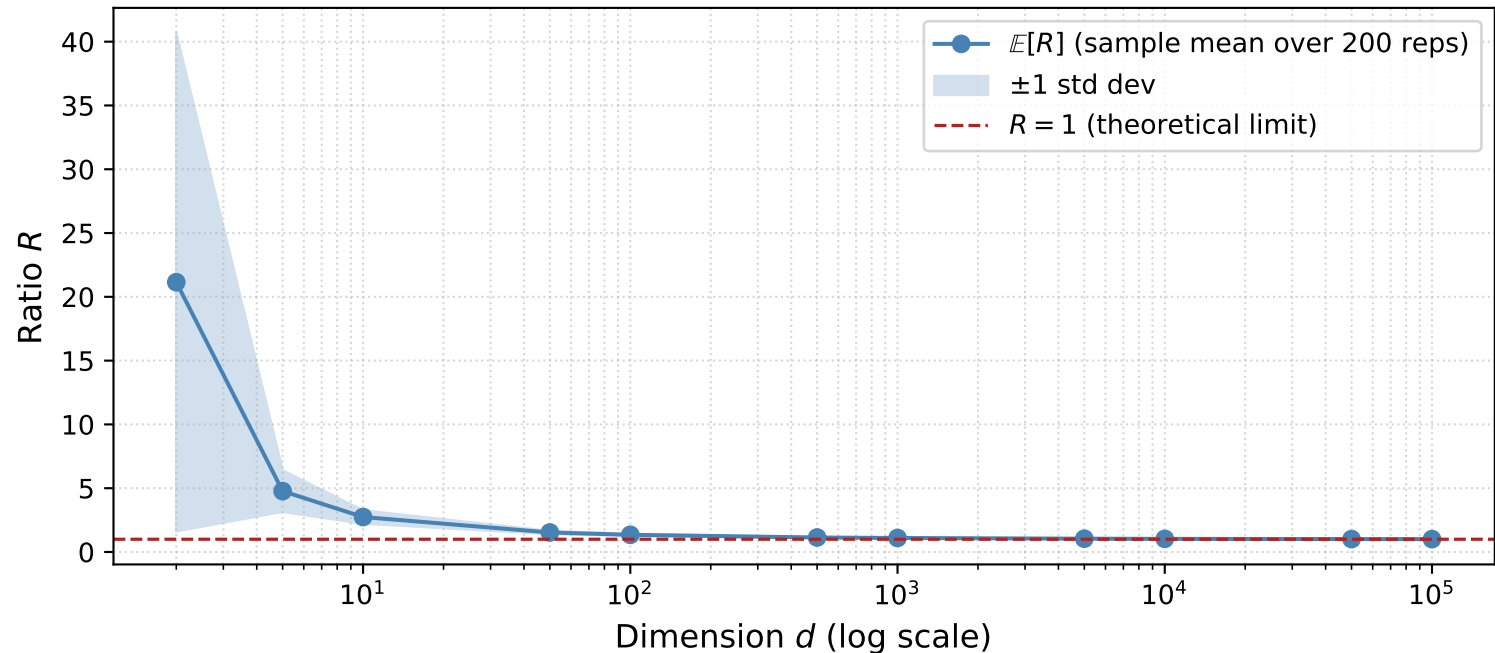
Ratio R = \max/\min pairwise distance for X_1, \dots, X_{10} \sim N_d(0, I_d)
